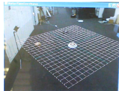
Fig. 5. Floor-Plane Construction by the 3D Posture of the Marker on the Robot
