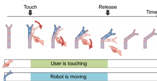
図6 Move-during-touch
