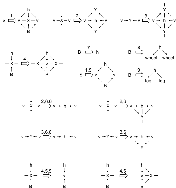
Figure 1: An example set of augmented rules. These are generated from Figure 2 (of the main paper) and following the description in Section 3.2.1 (of the main paper).
